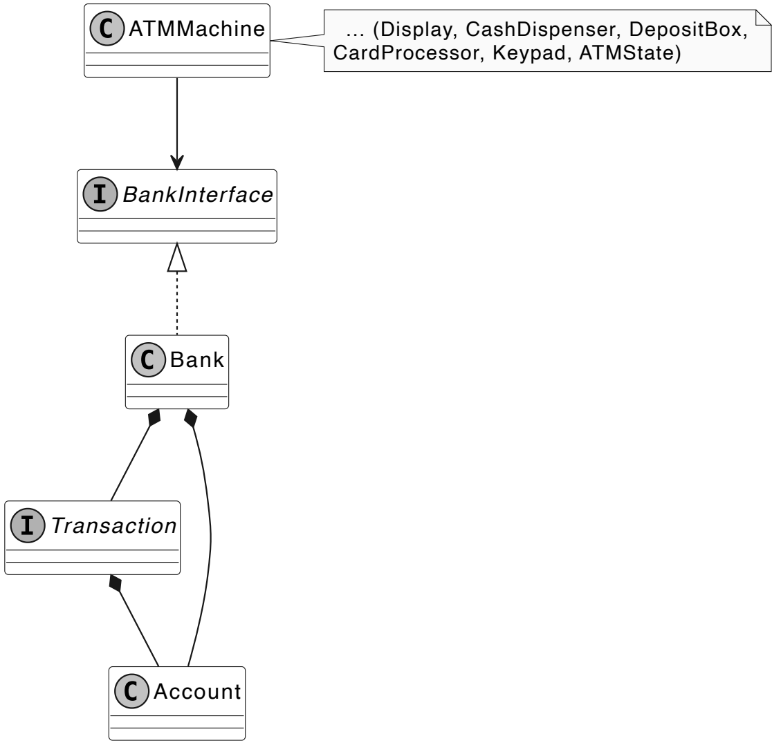
Summarized Class Diagram of ATM System
