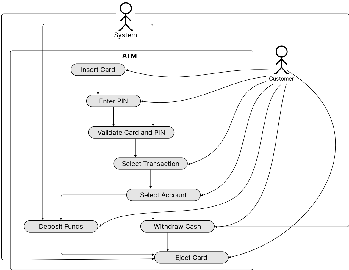
Use Case Diagram of ATM
